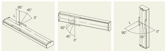
線性滑軌20x15.5-2支 (Linear Guide20x15.5-2 支)
